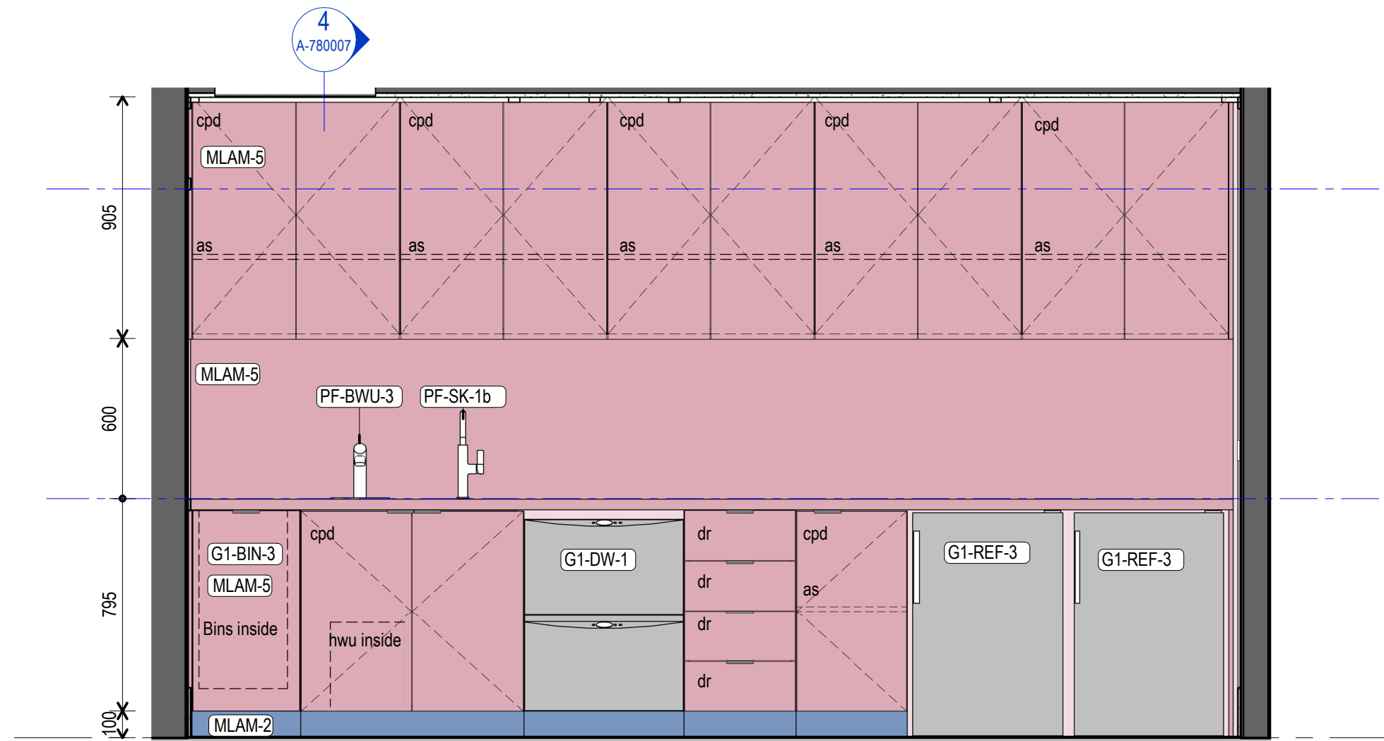
3 JO-BW-5 Elevation 1 : 20
